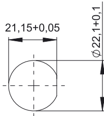
Drilling diagram
