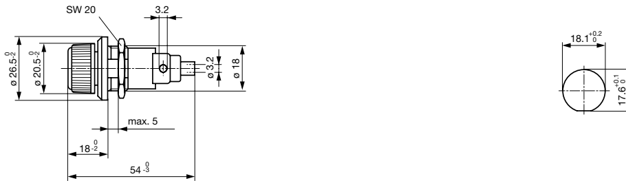
Mounting holes
