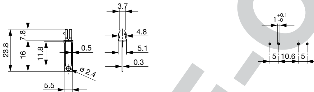
Drilling diagram
