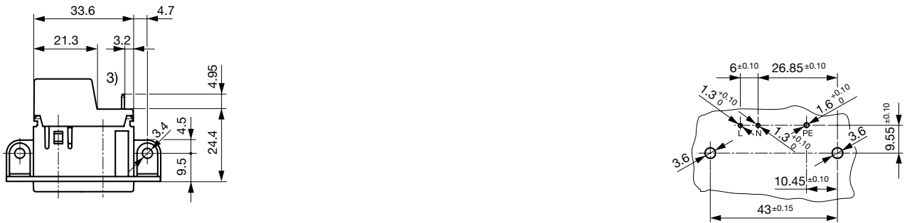
3) PE additionally as quick-connect terminal 4.8 x 0.8 mm
