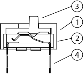
CONSTRUCTION
