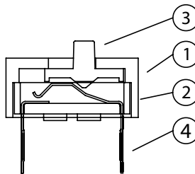
CONSTRUCTION
